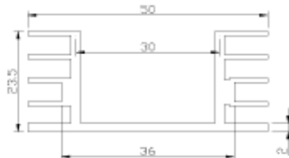
SRX-YC HEAT-SINK SECTION DIMENSIONS
